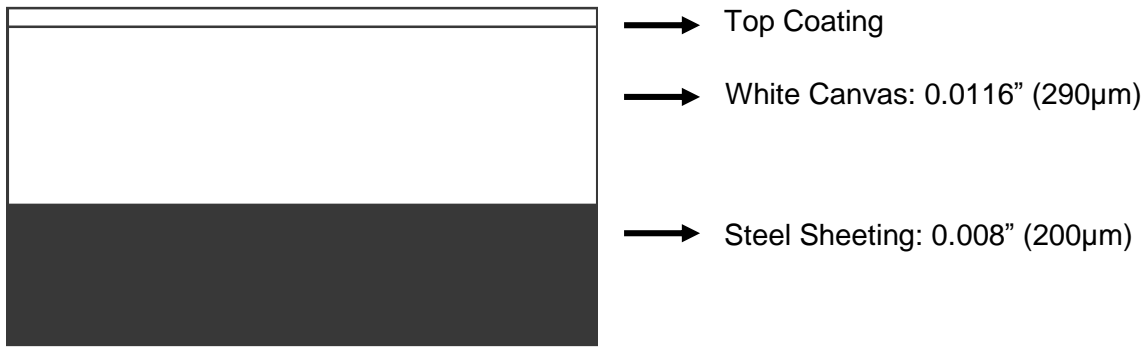
Construction Drawing
